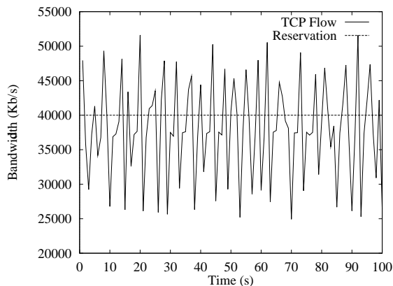
Figure 1: An application using TCP has made a reservation for only 40 Mb/s, when it is sending at 50M b/s.
