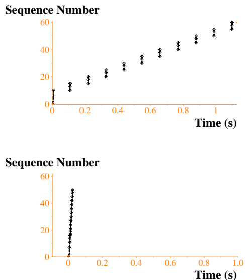
Figure 7: TCP traces of two programs that each send at 400Kb/s, but with very different burstiness characteristics. On the top is a program sending 10 frames per second, and each frame is 40Kb. On the bottom is a program sending just 1 frame per second, and the frame is 400Kb. (This corresponds to the first line of Table 1.) In each case, only one second of the program’s execution is shown.
