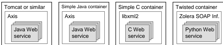
Figure 6: Four different GT4 container configurations.
