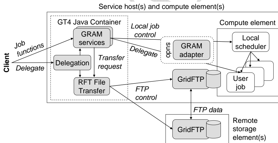
Figure 10: GRAM implementation structure
