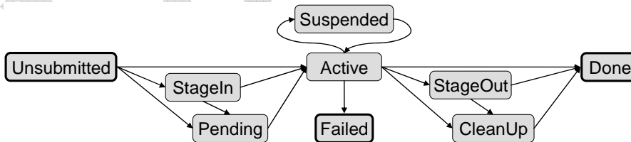
Figure 8: State transition diagram for GRAM jobs.
