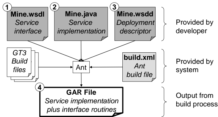
Figure 7: A Java Web service and the various components (shaded) that Axis uses to implement its interface and describe its configuration.
