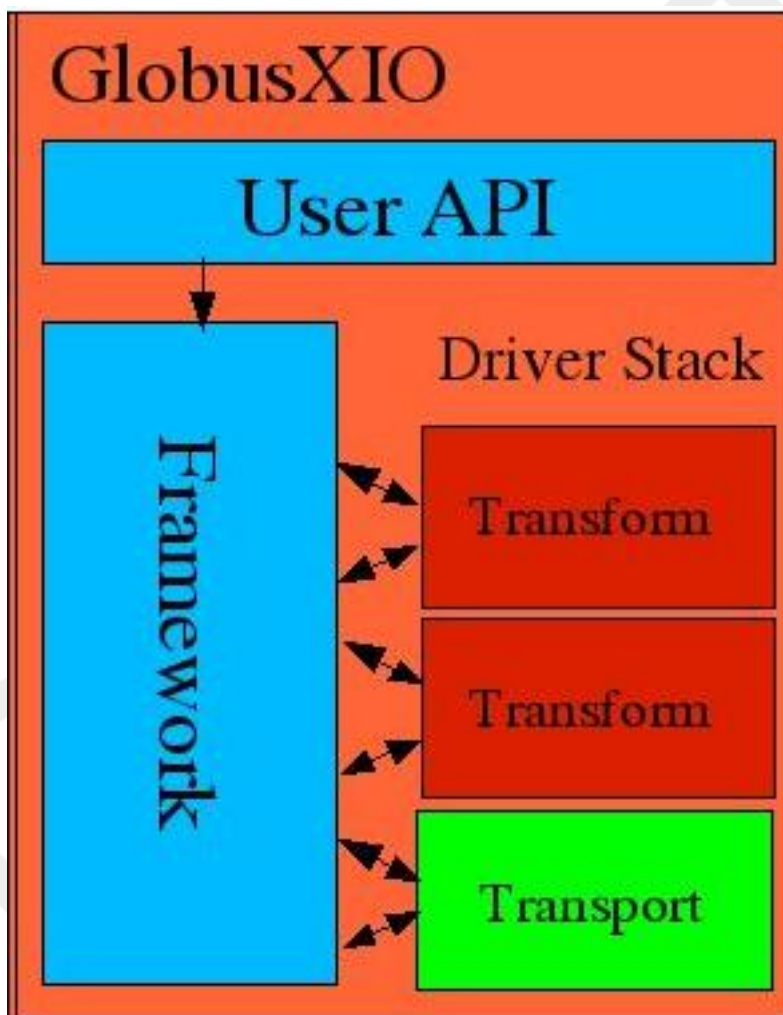
Figure 5.1. XIO Architecture
